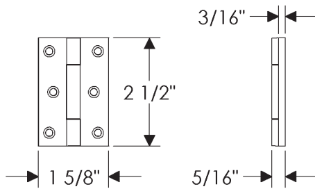
CABHNG420 Cabinet Hinge (Mortise) 2 1/2" x 1 5/8"
