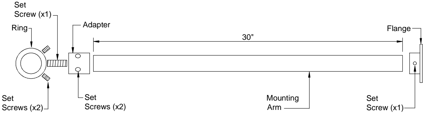
Exploded View
