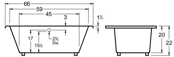
All bathtub dimensions are ± 1/2"
